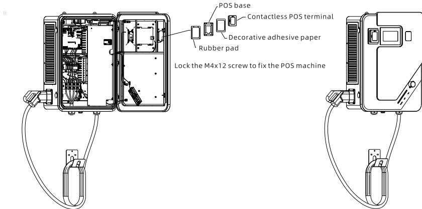
Step3: Contactless POS Terminal installation
