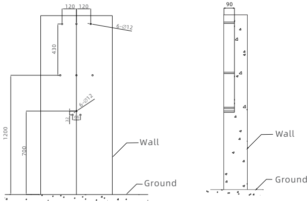
Drill holes on the wall
