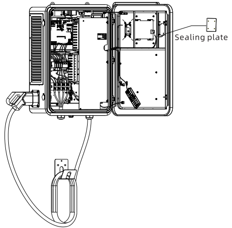
Step 2: Remove the sealing plate
