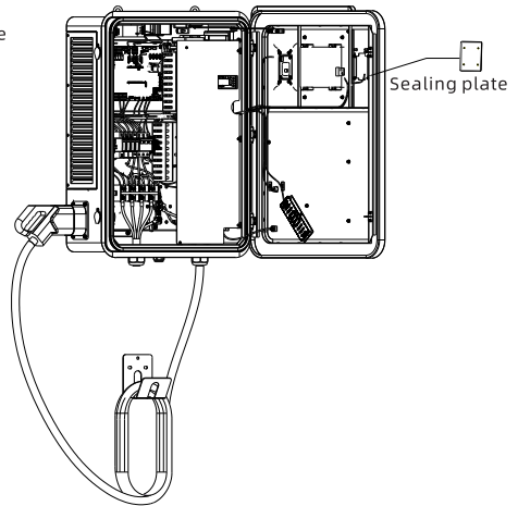
Step 2: Remove the sealing plate
