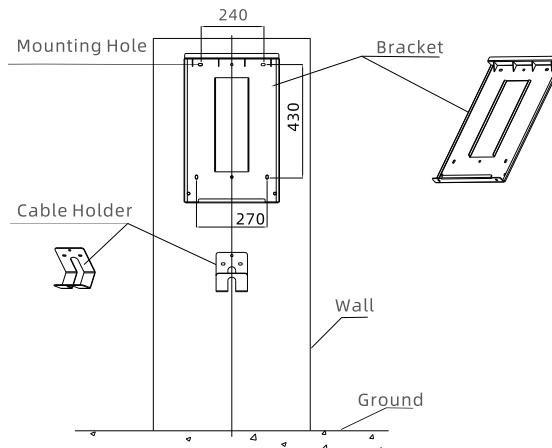
Mount the bracket and cable holder
