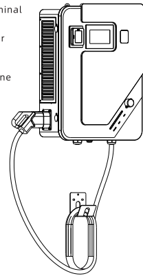
Step 4: Installation completed
