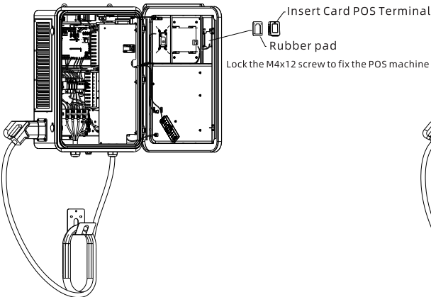
Step3: Insert Card POS Terminal installation
