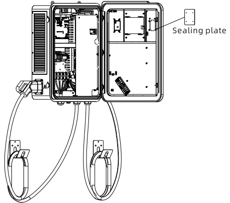
Step 2: Remove the sealing plate
