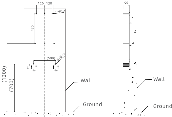
Drill holes on the wall
