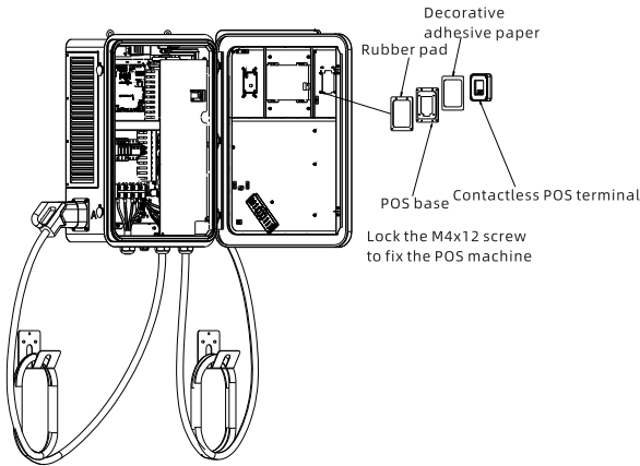
Step3: Contactless POS Terminal installation
