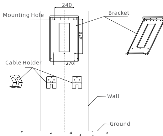
Mount the bracket and cable holder
