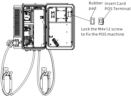
Step3: Insert Card POS Terminal installation
