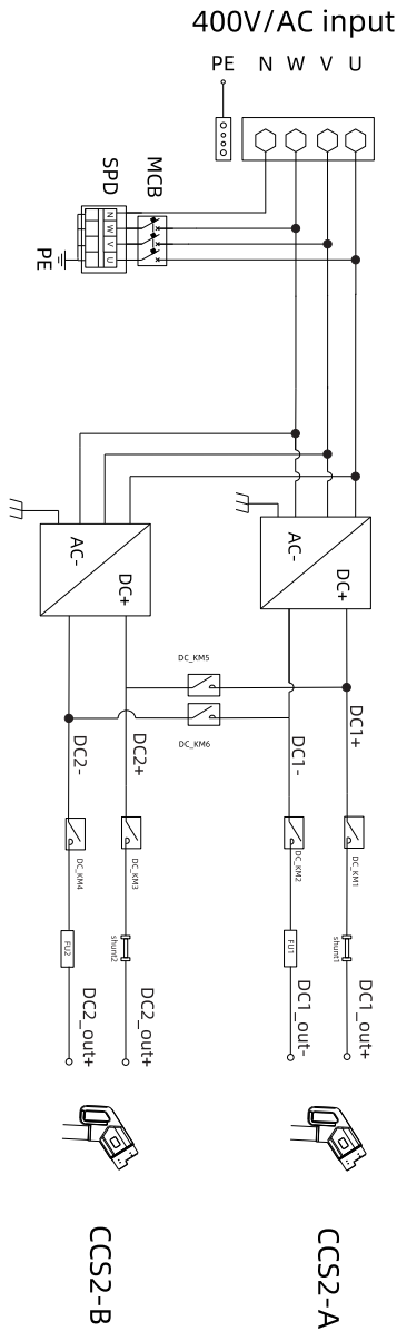
Fig7-2, Main circuit diagram
