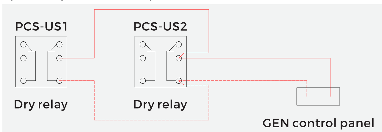
Dry Contact Diagram - PCS-US Parallel System
