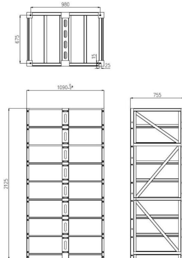
Figure 4 8 layers 2columns battery rack-1C size drawing
