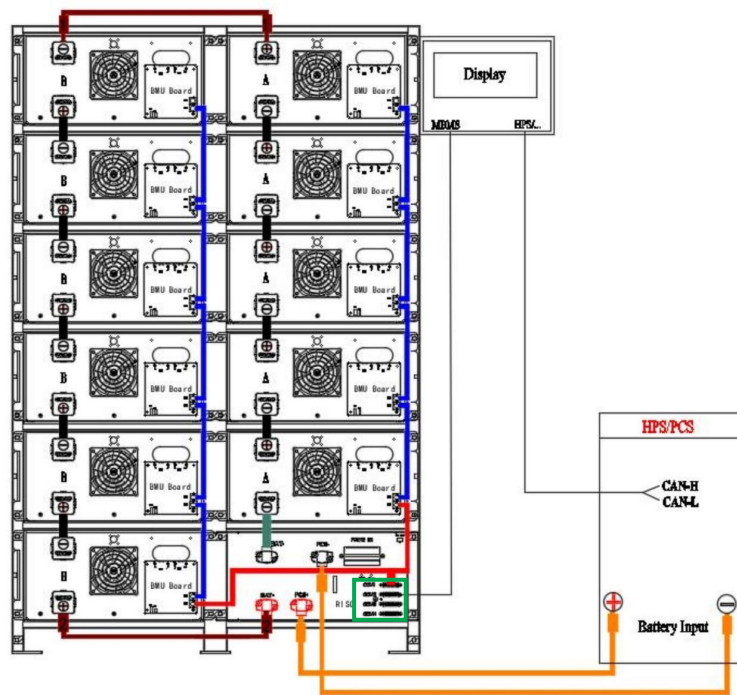
Figure 15 Battery energy storage system BPU-0.5C wiring diagram
