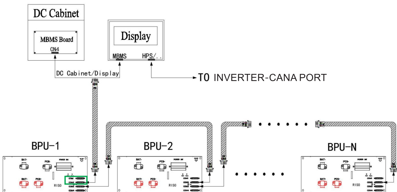
Figure 16 Battery energy storage system BPU-0.5C wiring diagram
