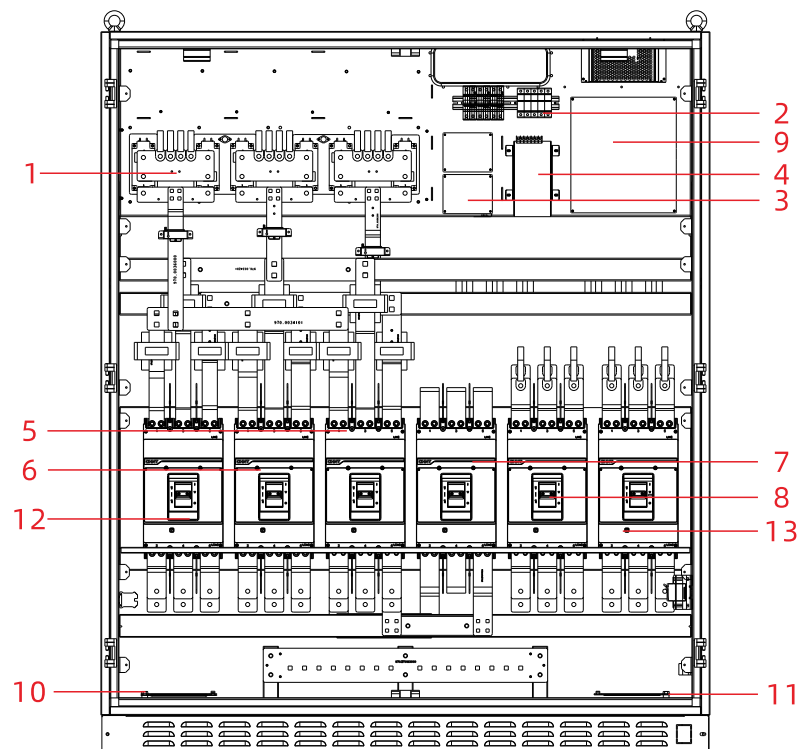
The front structure drawing of Bypass500/630-US
