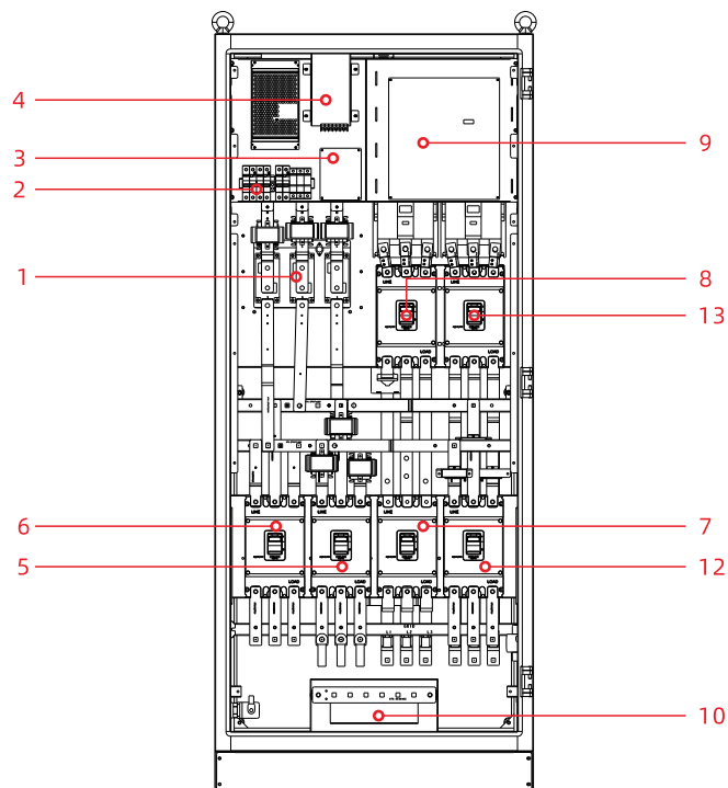
The front structure drawing of Bypass 250-US
