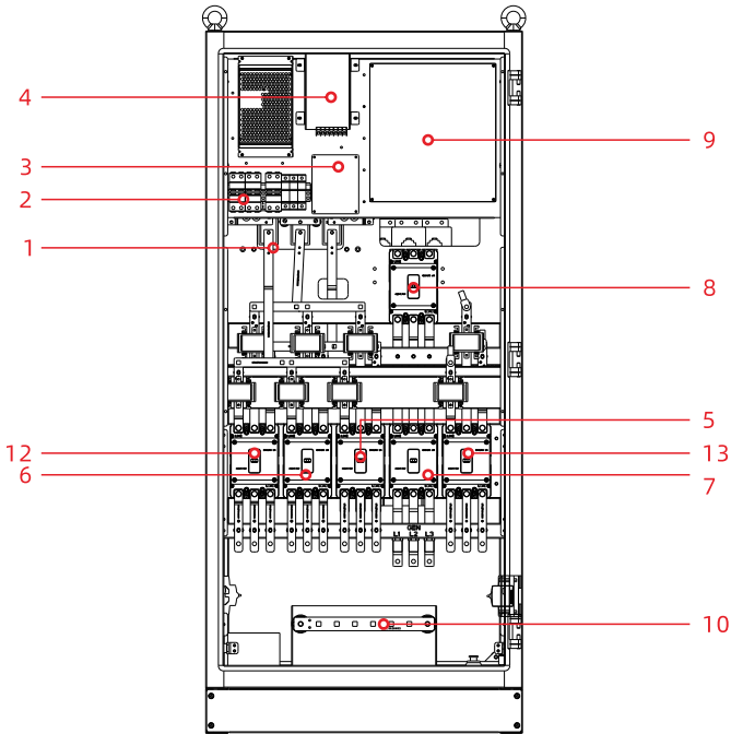
The front structure drawing of Bypass100-US
