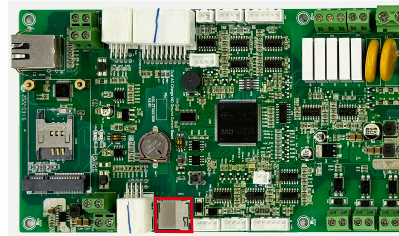
Micro SD slot of dual output charger
