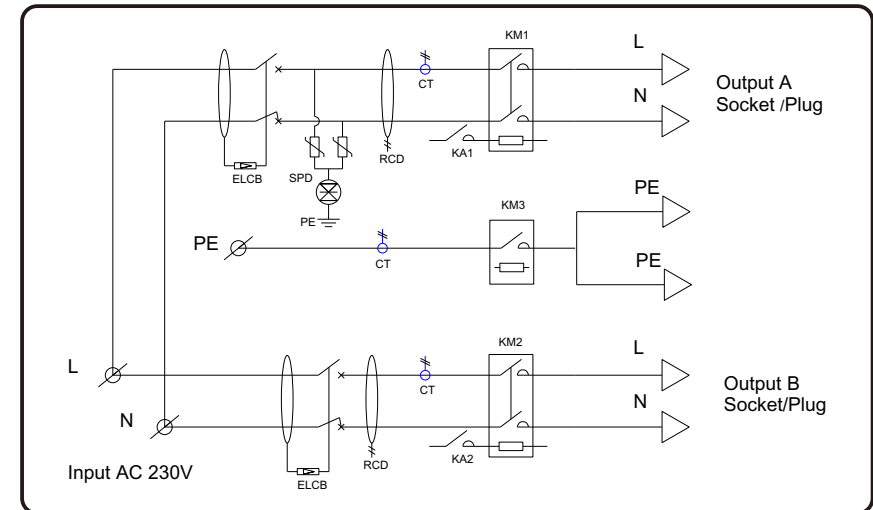
Fig11-1. Main circuit diagram
